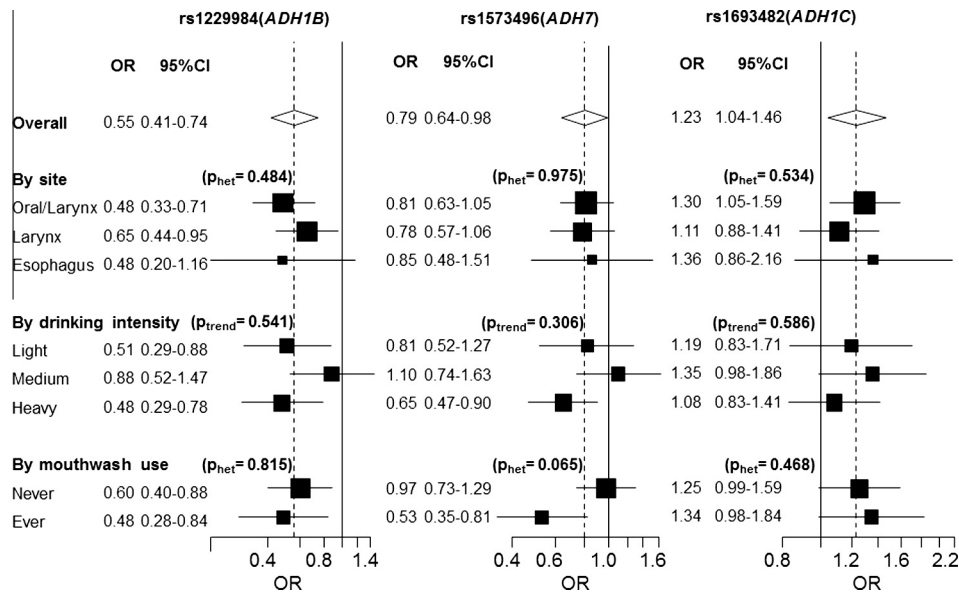
Figure 1. Odds ratio (OR) of upper aero-digestive cancer by rs1229984 (ADH1B), rs1573496 (ADH7) and rs1693482 (ADH1C) genotype. Rare allele carriers (dominant model) versus common allele homozygous genotype. ORs are standardized by age, sex, centre, cumulative alcohol consumption and, when relevant, smoking. P values for heterogeneity are derived from a Chi Square statistic with 2df. P values for trend test are derived from a Chi Square statistic with 1df.
